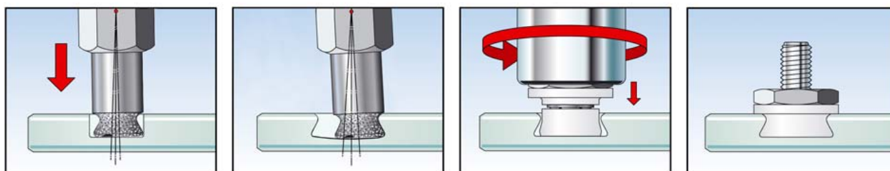
Drilling and anchor setting procedure for the FZP-G-Z point holder in glass
