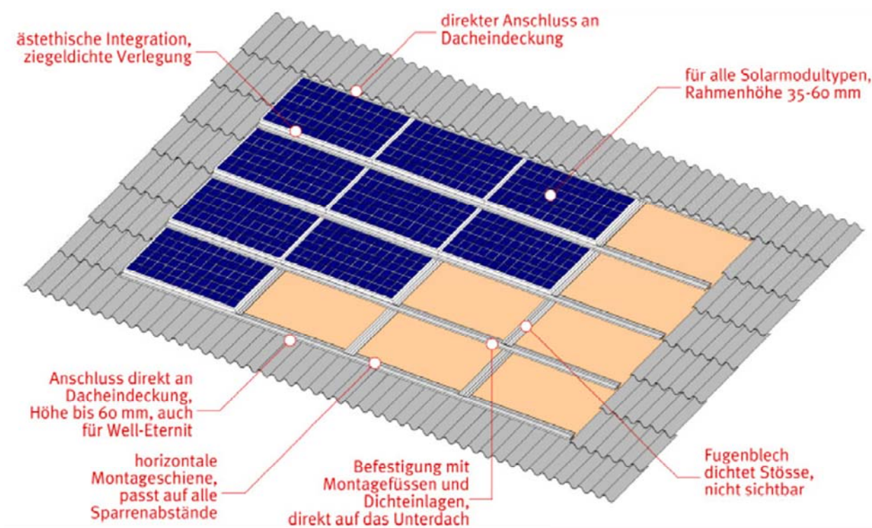
Fixing system scheme
