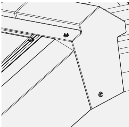
Ridge detail
