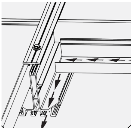
Sealing ducts
