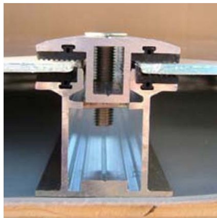
Panel connecting section
