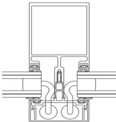
Section of the support
