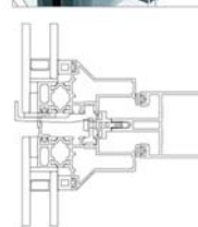
System and section of "Elegance 52 SG TH"
