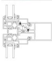
System and section of "Elegance 52 GF"
