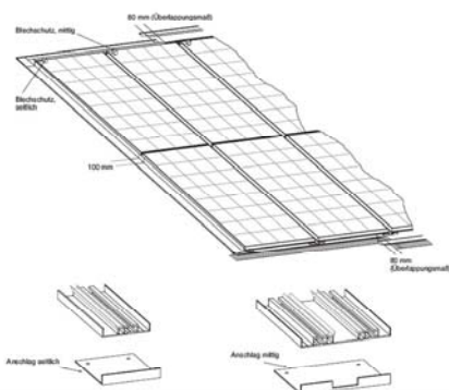
Support and position of the panels
