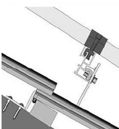
Fixing detail
