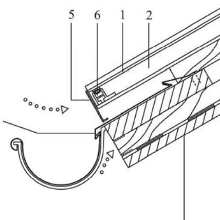
Gutter section
