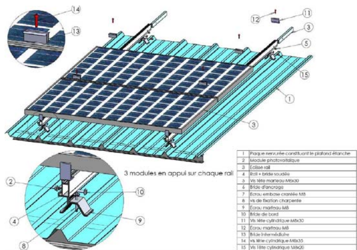
Profile of fastening system
