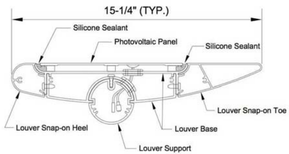
LOUVER CROSS SECTION WITH PHOTOVOLTAIC PANEL
